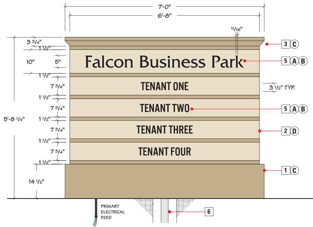
1 FRONT VIEW SCALE: 1/2" = 1' - 0" 39.8 SQ. FT.
